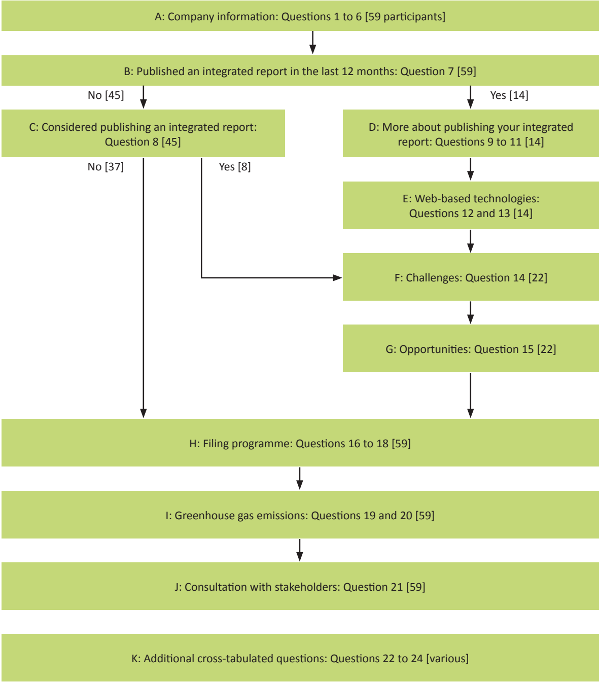
Figure 2: Survey Logic
