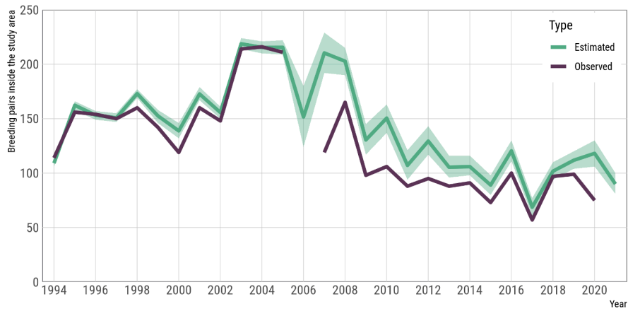
Figure 8: Comparison of the annual number of breeding pairs when recorded during field surveys (Observed) and when estimated from the model (Estimated). Lines indicate the mean, shading the 95% credible interval for the estimate.
