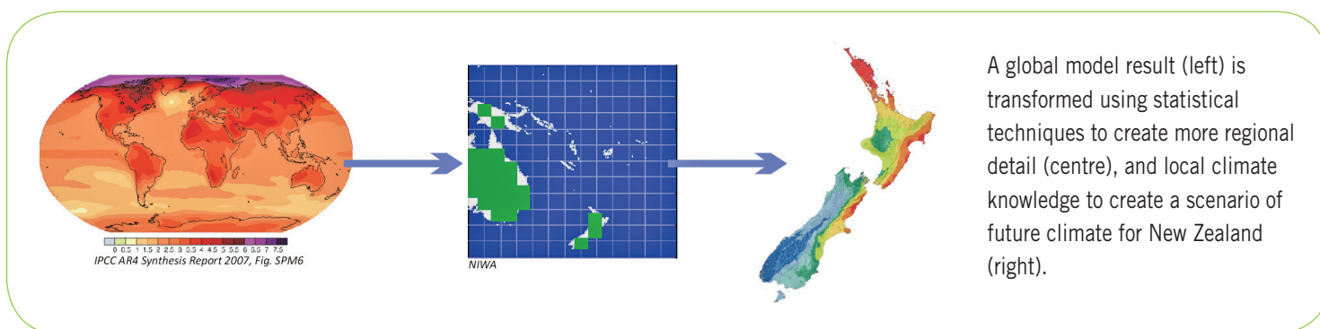
FIGURE 3: SCHEMATIC REPRESENTATION OF THE DOWNSCALING PROCESS
