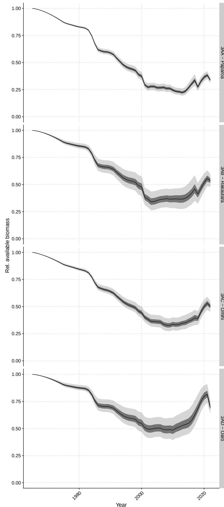
Figure D-9: Estimated relative available biomass trend for pāua for the base operating model, fitted to survey observations, including earthquake impacts modelled as instantaneous natural mortality (short term) and reduced recruitment (long term) proportional to uplift in each management zone in the model for quota management area PAU 3A (median line, inter-quartile range (dark shaded area) and 95% confidence interval (lighter shading)).
