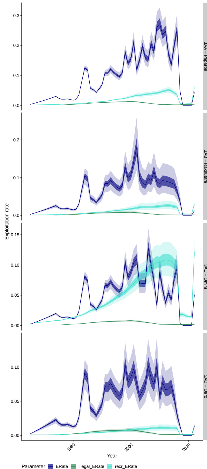
Figure D-11: Estimated exploitation rate (median line, inter-quartile range (dark shaded area) and 95% confidence interval (lighter shading)) for commercial (ERate), recreational (recr) and illegal components of the fishery in the base operating model, fitted to survey observations, including earthquake impacts modelled as instantaneous natural mortality (short term) and reduced recruitment (long term) proportional to uplift in each management zone in the model for quota management area PAU 3A.
