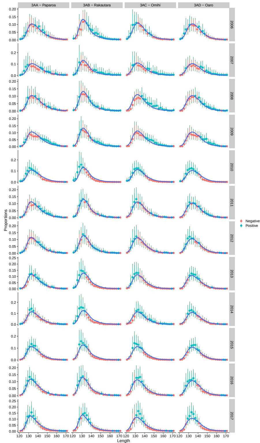
Figure D-5: Comparison of posterior mean predicted catch sampling length frequency (CSLF) with estimated CSLF proportions and observation error for the base operating model, fitted to survey observations, including earthquake impacts modelled as instantaneous natural mortality (short term) and reduced recruitment (long term) proportional to uplift in each management zone in the model of pāua for quota management area PAU 3A. Length classes with positive residuals in blue, with negative residuals in red.
