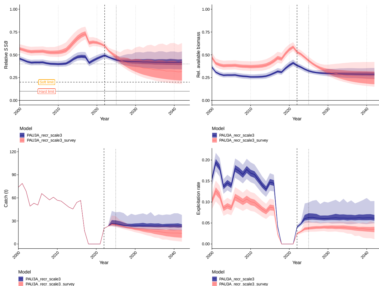
Figure 35: Projected relative spawning stock biomass ( SSB ), available biomass (at current minimum harvest size), long-term commercial catch and exploitation rate under two models for PAU 3A, fitted (or not) to survey observations, assuming rapidly declining recreational catch with available biomass (scale3).
