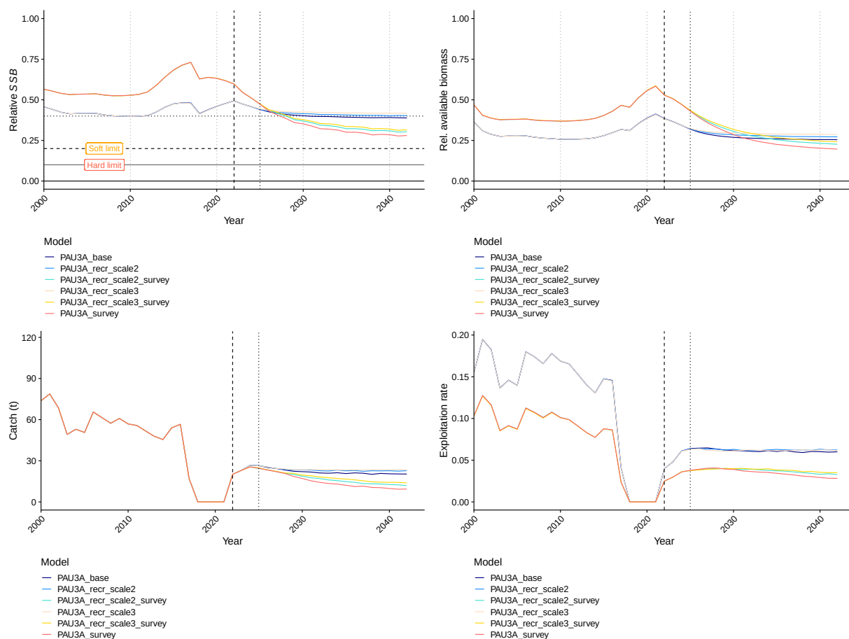
Figure 37: Projected relative spawning stock biomass (SSB), available biomass (at current minimum harvest size), long-term commercial catch and exploitation rate for models fitted to survey observations (_survey) or not for PAU 3A, using the model with maximum assumed earthquake impacts, and scaling recreational catch according to available biomass, either by scaling directly or as a square or cube of available biomass (scale2, scale3).
