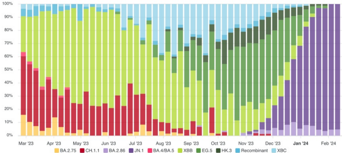
Figure 4: Change in the national percentage of variants per week over the last 12 months.
